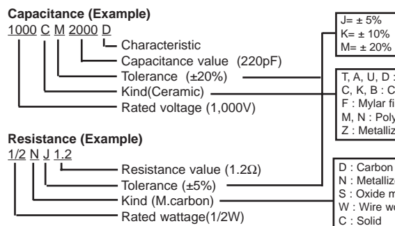
Expression of capacitance and resistance in circuit diagram.
